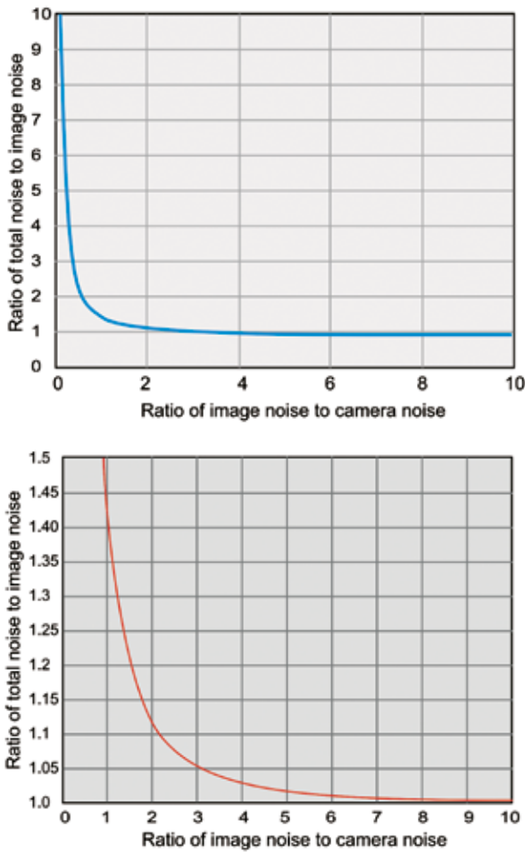
Figure 3 — Total-noise ratio versus image-noise ratio. The bottom image is a magnified view of around the inflection point of the top curve.
