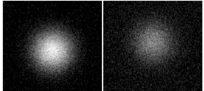
Figure 2 — A simulated star image showing its appearance at differing SNRs.
