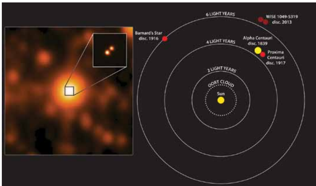
Figure 4 — Left: WISE 1049-5319 is at the centre of the larger image taken by WISE, the inset shows sharper image from Gemini Observatory (NASA / JPL / Gemini Observatory / AURA / NSF). Right: this diagram illustrates the locations of the star systems that are closest to the Sun (Janella Williams / Penn State University)
