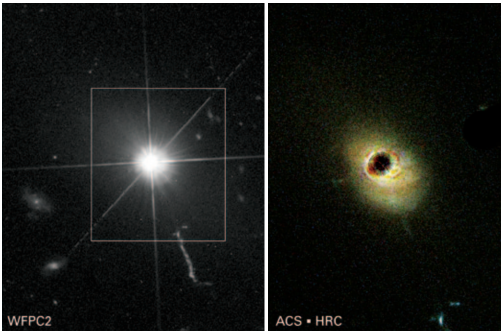
Figure 2 — The quasar 3C 273 is revealed in this pair of Hubble Space Telescope images, one (left) acquired by the older Wide-Field Planetary Camera 2, shows the brilliant quasar but little else. The diffraction spikes demonstrate the quasar is truly a point-source of light because the black hole’s “central engine” is so compact. The newer Advanced Camera for Surveys (ACS) coronagraph reveals features in the surrounding galaxy that are normally drowned out by the quasar’s glow. The ACS reveals a spiral plume wound around the quasar, a red dust lane, and a blue arc and clump in the path of the jet blasted from the quasar. Previously known clumps of hot gas and the inner blue optical jet are now resolved more clearly. Image: NASA and J. Bahcall (IAS).
