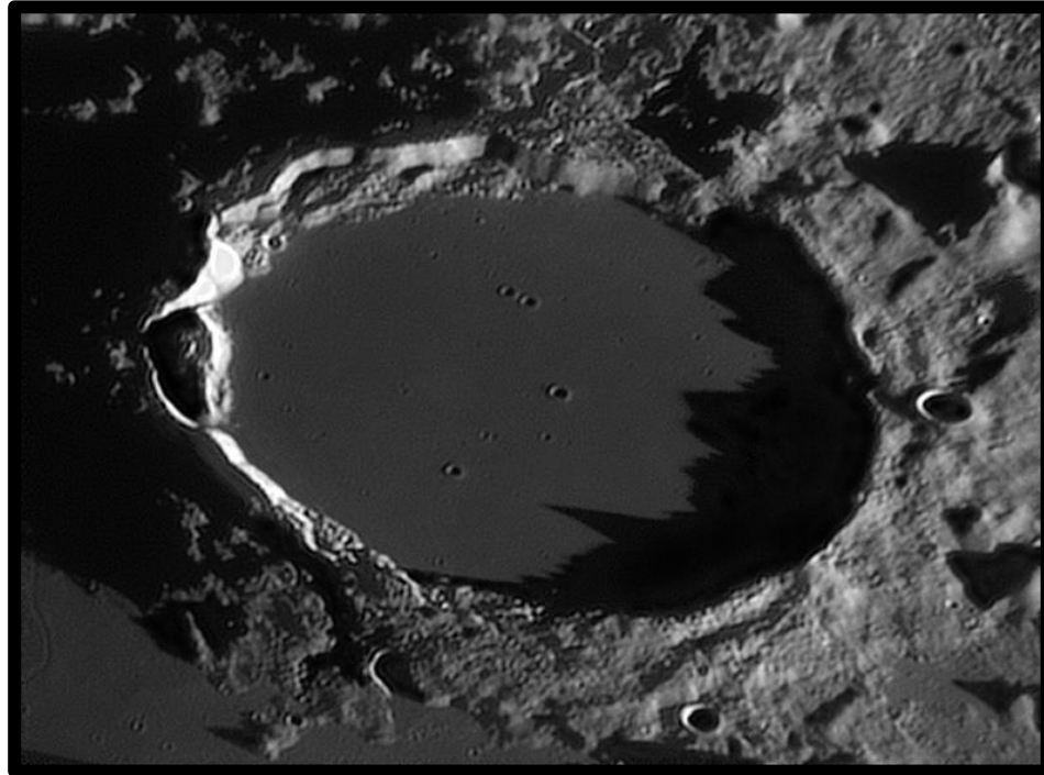
Crater Plato
