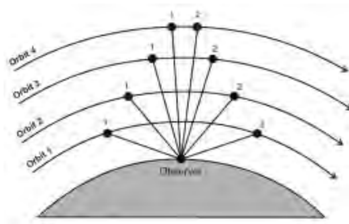
Figure 2 — Four satellites in four different orbits seen by an observer at the zenith. The observed angular velocities will depend on both the satellites' distances from the observer and the satellites' linear velocities, as stated in Equation 1.
