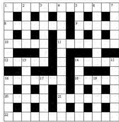
Astrocryptic p. 236
