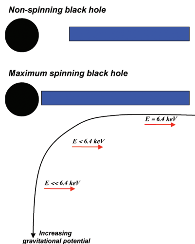
Figure 12 — The inner edge of the accretion disc extends closer to the black-hole event horizon as the black hole spins. Photons emitted closer to the black hole climb out of a deeper gravitational potential well and lose more energy in the process — they are gravitationally redshifted.
