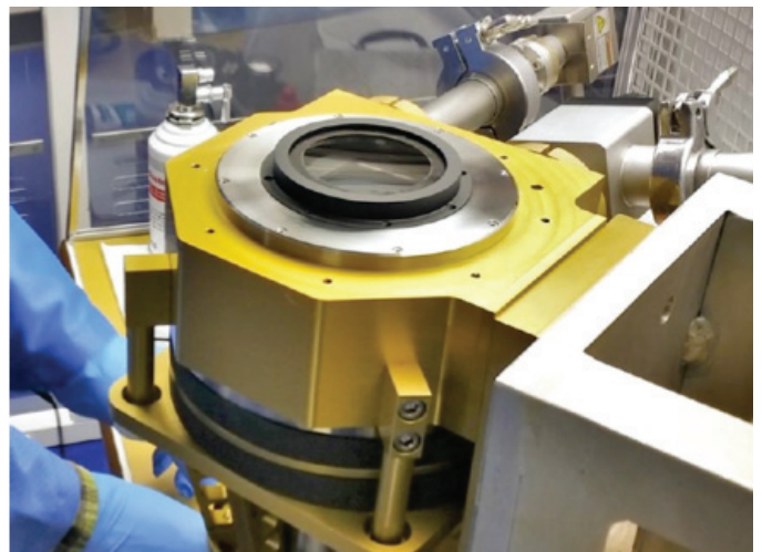
Figure 2 – Installation of the SITELLE corrector lenses on the cryostats
